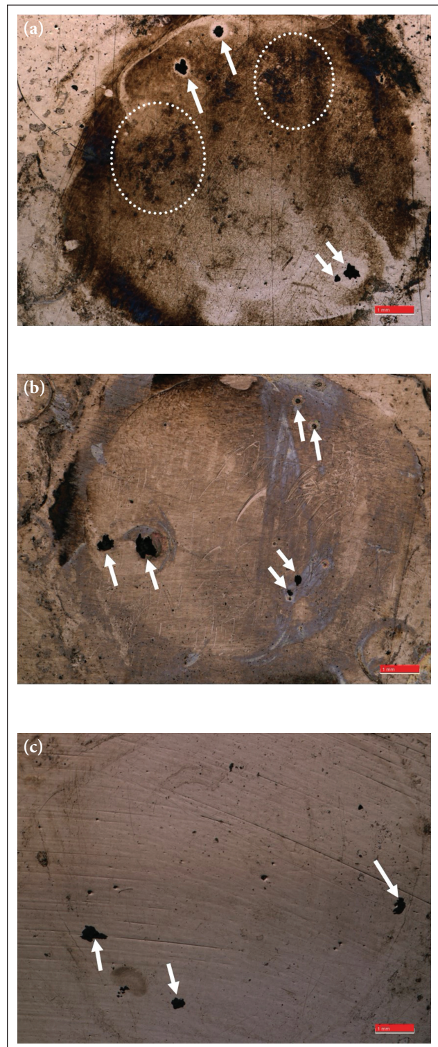
Figure 3. Surface microstructure of the samples after PDP tests (a) in 3.5% NaCl, (b) in 3.5% NaCl + 1% \text{NH}_4\text{NO}_3 , and (c) 3.5% NaCl + 3% \text{NH}_4\text{NO}_3 .
