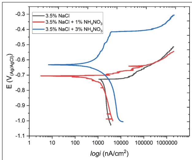
Figure 2. Potentiodynamic polarization curves.
