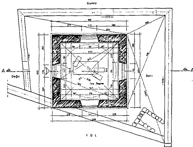
PLAN 1/50
