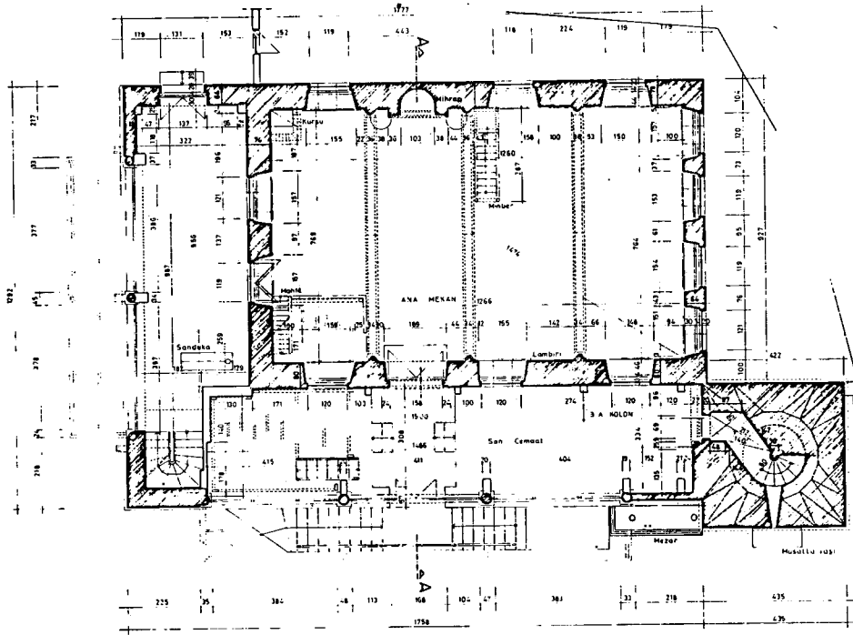
Plan 1/50
