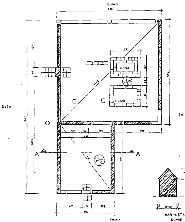
PLAN 1/50
