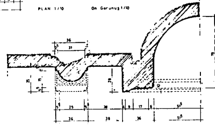
KEMER ve MİHRAP DETAY PLAN 1/10
