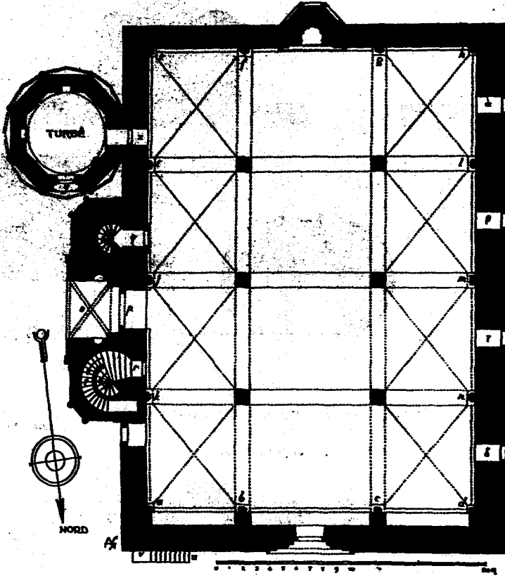
Fig. 77. — Mosque at Sungurbey. Plan (reduced).
